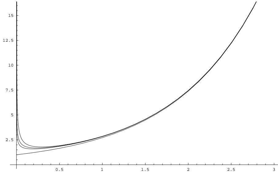
Figure 2.4: Riemann-Liouville fractional derivatives of f(x) = e^x with base point at a = 0 for \alpha = 0, 1/2, 1/3, 1/4 . Observe how at small x the x^{-\alpha} term dominates the Mittag-Leffler function.
