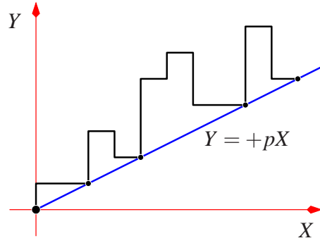
Figure 3: A bargraph path above the line Y = +pX . The generating function of this model is not known explicitly. However, a set of equations derived in reference [26] can be solved to determine the radius of convergence of the generating function for integer values of p .
