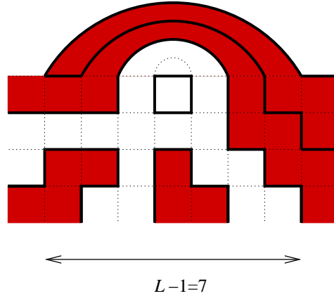
Fig. 17. A HTSFPL diagram of size (2n-1) \times n = 7 \times 4 with link pattern ) \cdot (\cdot) \cdot (\cdot) \cdot ((\cdot) , having three nests.
