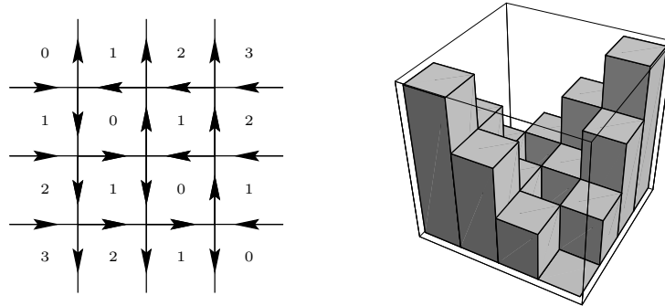
Fig. 5. Vertex and height interpretation corresponding to the 3 \times 3 identity matrix.
