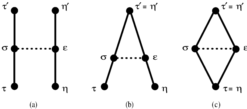
FIGURE 2. A pair (\tau\sigma\tau', \eta\varepsilon\eta') of joined 2-paths: (a) type H; (b) type A; (c) type \theta .
