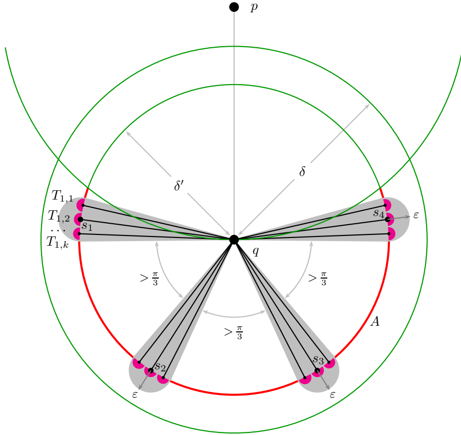
FIGURE 4. Construction in the proof of Lemma 3.3.
